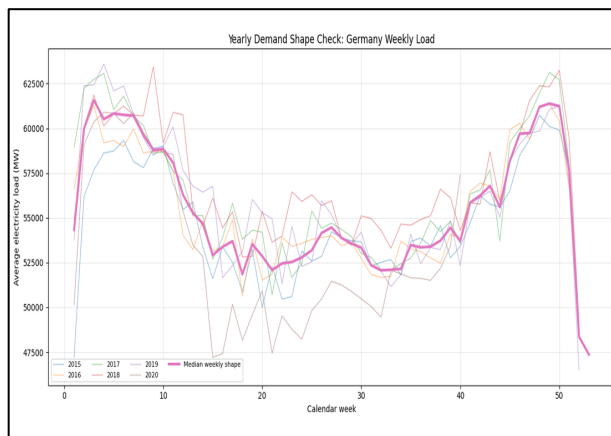
Figure 1. Weekly demand shape by calendar week.
